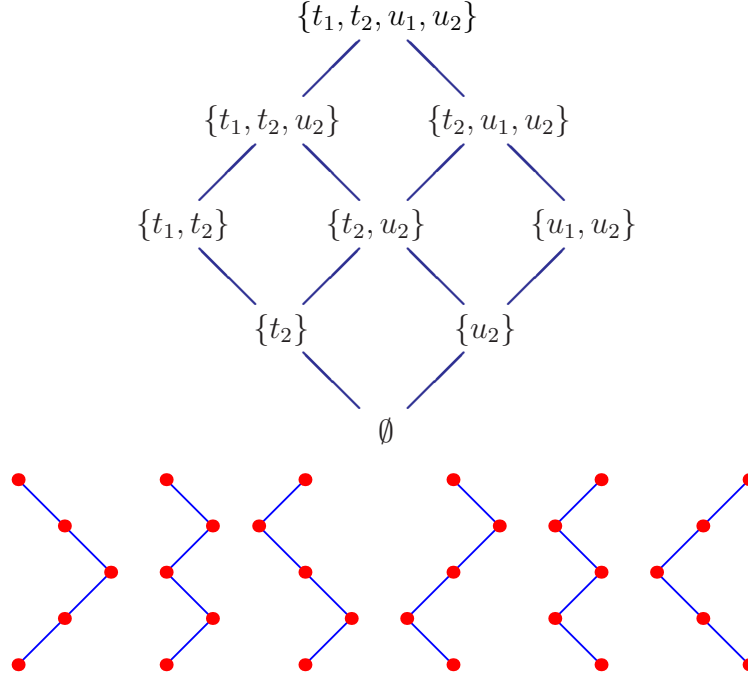
FIGURE 4. The distributive lattice \mathcal{J}(P) and its maximal chains.
