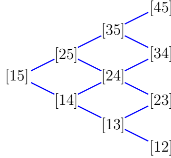
FIGURE 7. The distributive lattice \mathcal{C}_{2,3} .
