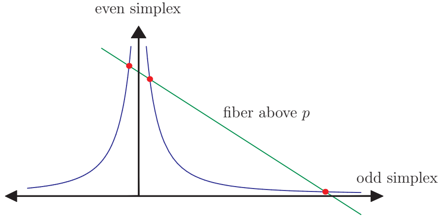
FIGURE 3. Preimages near coordinate spheres.
