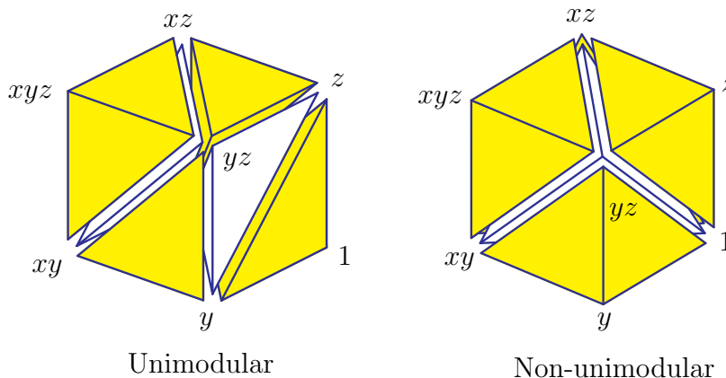
FIGURE 6. Triangulations of Cubes
